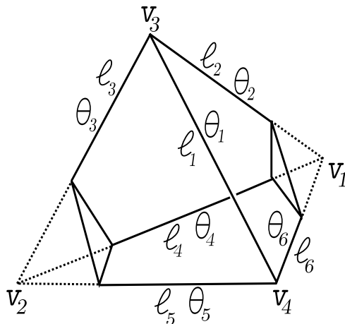
Figure 1: Mildly (doubly) truncated tetrahedron
