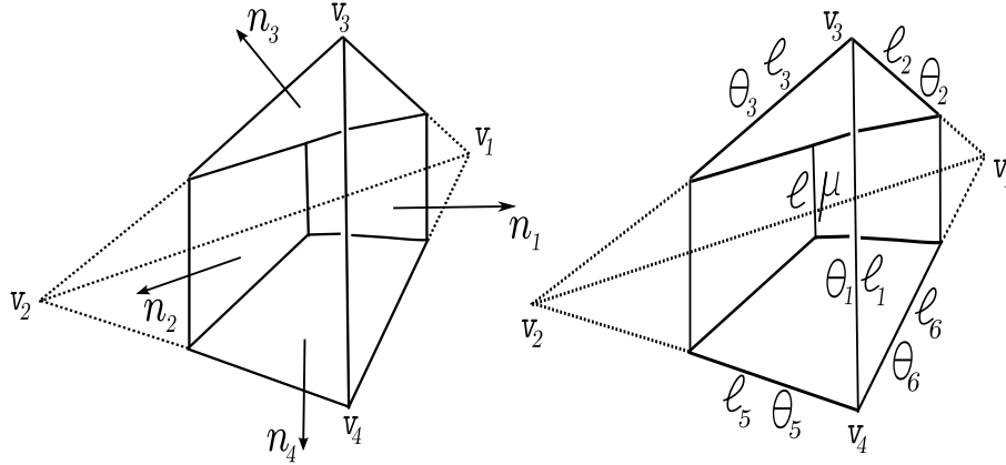
Figure 2: Prism (intensely) truncated tetrahedron T and its geometric parameters
