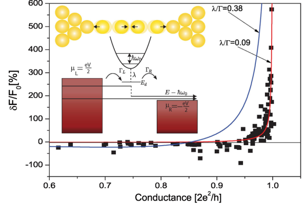
FIG. 3 (color online). Distribution of the observed change in the Fano factor at the kink, plotted as a function of the conductance. The points are obtained for different realizations of Au atomic chains. For conductance (i.e., transmission) close to 1 we find exclusively positive values for \delta F/F . Below a cross-over regime near G = 0.95G_0 only negative values are observed. The curves are obtained from the theory of Ref. [9], for fixed values of the inelastic scattering strength \lambda . Inset: The top part illustrates the atomic chain configuration and the vibration mode involved in the scattering. The lower part sketches an example of a two-electron process giving rise to reduction of the Fano factor: two electrons injected from the left lead at different energies tend to compete for the same outgoing state after the emission of a phonon (see text).
