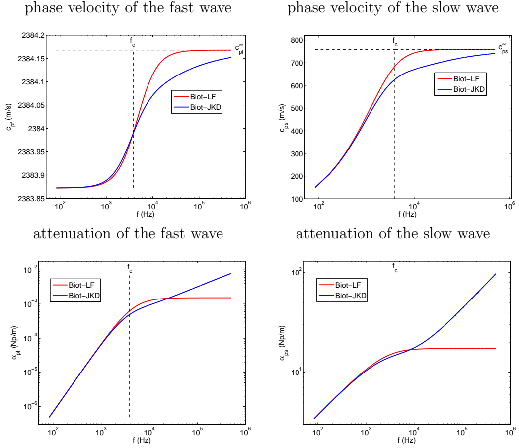
Figure 1: Dispersion curves: comparison between Biot-LF and Biot-JKD.
