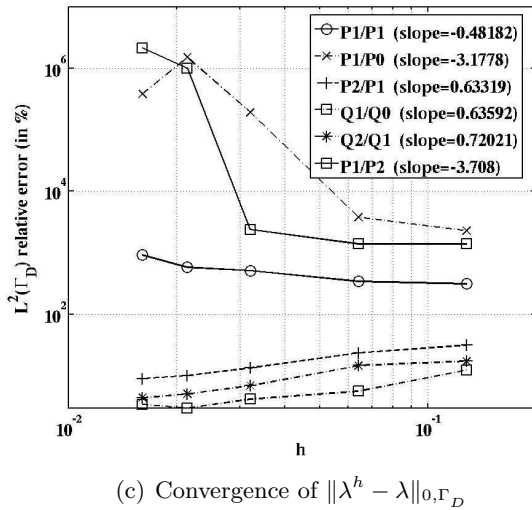
Figure 15: Convergence curves in the three-dimensional non-stabilized case.
