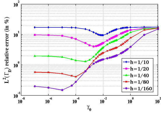
Figure 14: Influence of the stabilization parameter for the error in in L^2(\Gamma_D) -norm of the multiplier for the P_2/P_1 -elements (with a minimal patch size equal to h ).
