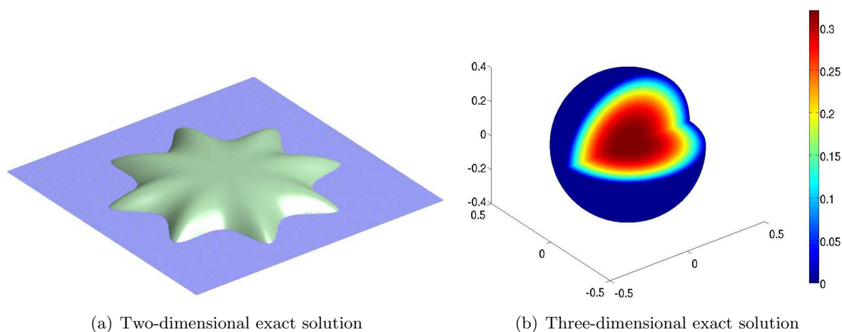
Figure 5: Exact solutions
