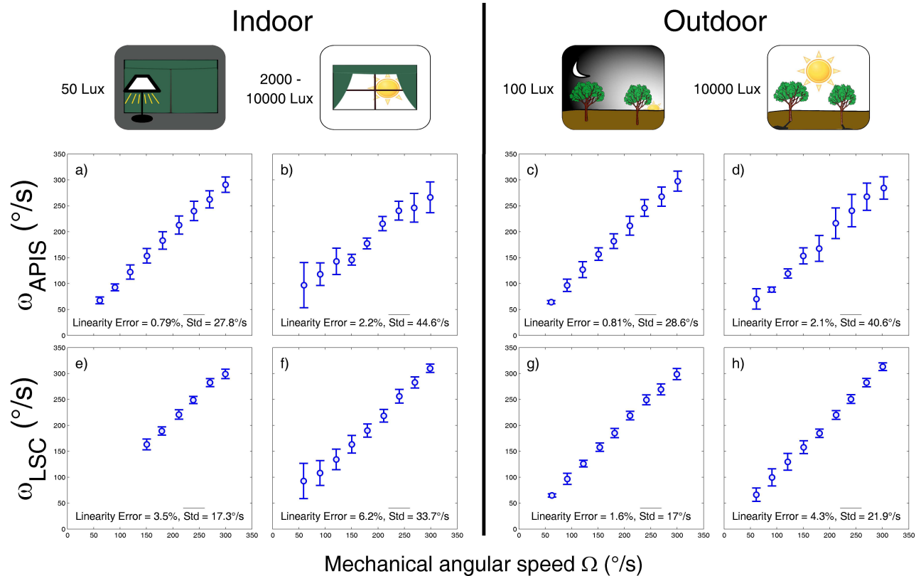
Figure 5: Static indoor and outdoor characteristics of the LSC- and APIS-based local motion sensors assessed by applying 30^\circ/s steps (lasting 15 seconds) to the rotational speed from 60^\circ/s to 300^\circ/s . The background illuminance ranged indoors between 50lux and 2000lux (apart from some peaks at 10000lux) and outdoors between 100lux and 10000lux. The mean visual motion recorded at each angular speed \Omega is plotted in this figure with its standard deviation. The best linear approximation obtained in each experiment was computed and the departure from linearity is given as a percentage.
