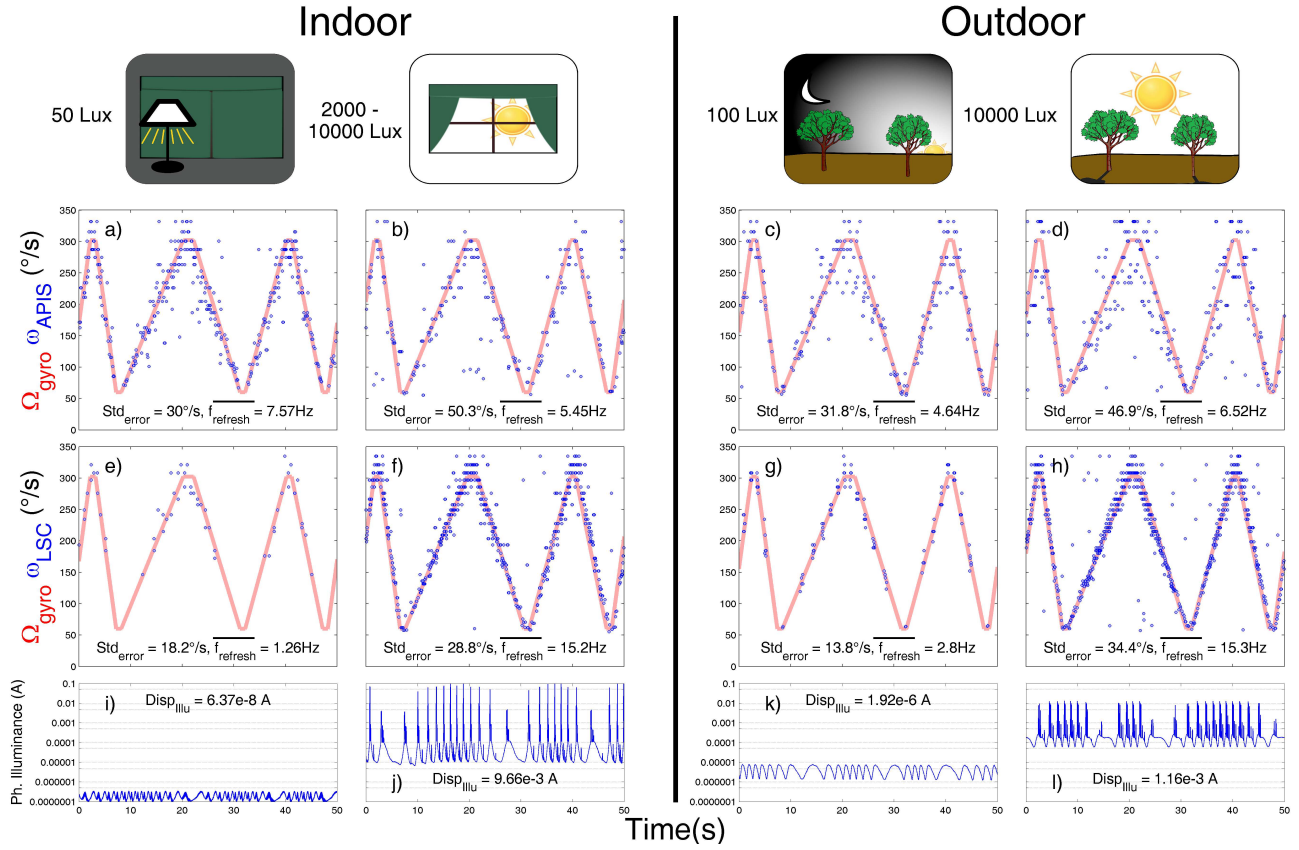
Figure 7: Dynamic indoor and outdoor responses of the two visual motion sensors (blue dots, figure 4a and 4b). The visual motion sensors mechanically rotated, giving a triangular pattern of angular speed variation (red) involving a series of velocity ramps ranging between 60 ^{\circ}/s and 300 ^{\circ}/s with different slopes under four different lighting conditions. Despite the strong illuminance variations, both visual motion sensors followed the rotational angular speed quite faithfully. With both sensors, the error between the measured local motion \omega_{meas} and the angular velocity measured by the rate gyro \Omega_{gyro} was used to compute the standard deviation of the error. The average refresh rate of the sensor was defined here as the number of new measurements occurring during the whole experiment divided by the duration of the experiment.
