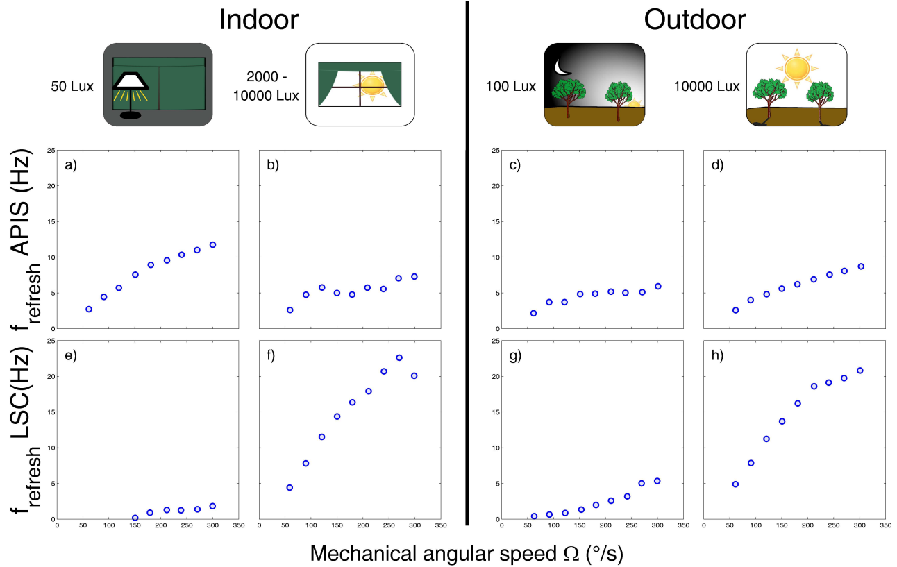
Figure 6: Refresh rates of the LSC- and APIS-based local motion sensors measured indoors and outdoors at a rotational speed ranging from 60^\circ/s to 300^\circ/s in 30^\circ/s steps (lasting 15s).
