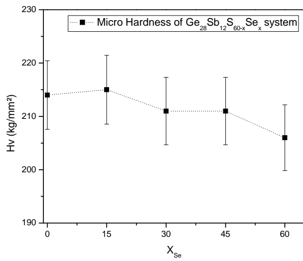
Figure 4: Evolution of the micro-hardness as function of the substitution of S by Se in \text{Ge}_{28}\text{Sb}_{12}\text{S}_{60-x}\text{Se}_x glass system. Static load equals 10 mN. Errors bars shown are \pm 3\% .
