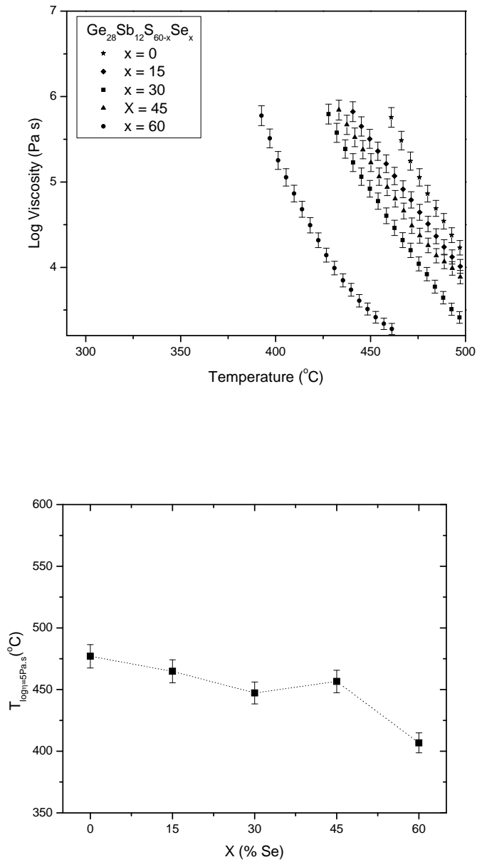
Figure 6: a) Evolution of the transition range viscosity behavior in the \text{Ge}_{28}\text{Sb}_{12}\text{S}_{60-x}\text{Se}_x glass system as a function of Se content (x, mol%). b) Evolution of the drawing temperature of \text{Ge}_{28}\text{Sb}_{12}\text{S}_{60-x}\text{Se}_x glass system as function of Se content (x, mol%).
