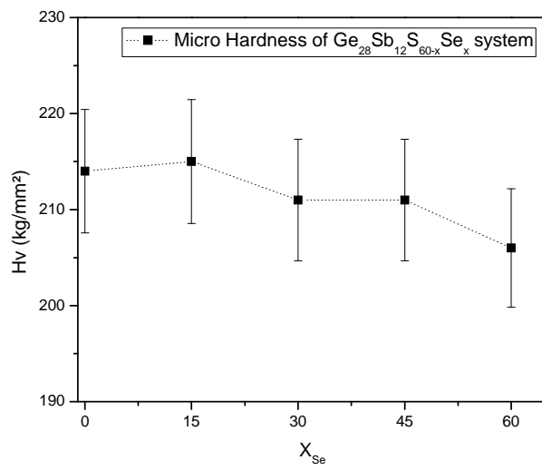
Figure 4: Evolution of the micro-hardness as function of the substitution of S by Se in Ge_{28}Sb_{12}S_{60-x}Se_x glass system. Static load equals 10 mN. Errors bars shown are \pm 3\% .
