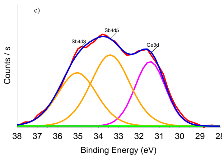
Figure 3: High resolution XPS spectrum of Ge3d levels for the investigated a) \text{Ge}_{28}\text{Sb}_{12}\text{S}_{60} , b) \text{Ge}_{28}\text{Sb}_{12}\text{S}_{30}\text{Se}_{30} and c) \text{Ge}_{28}\text{Sb}_{12}\text{Se}_{60}
