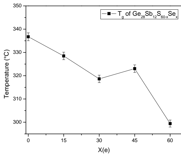
Figure 5: Evolution of the glass transition temperature T_g as function of the substitution of S by Se in glass system.
