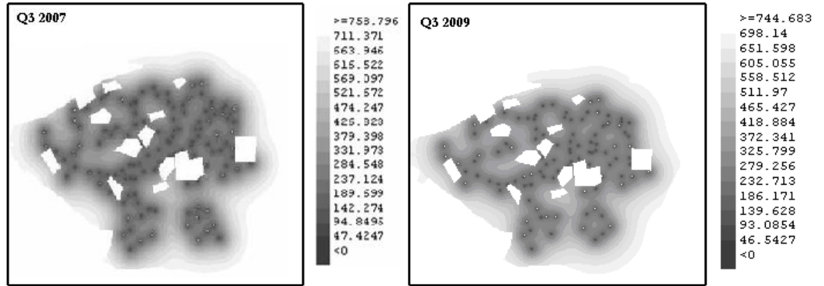
FIGURE 4: Standard deviation corresponding to the cokriged valuation of the commercial property prices. Maps corresponding to Q3 2007 and Q3 2009.
