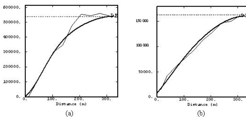
FIGURE 2: Experimental and fitted (a) premises prices direct variogram Q3-2007, (b) house prices direct variogram Q3-2007, (c) premises prices-house prices cross-variogram Q3-2007, (d) premises prices direct variogram Q3-2009, (e) house prices direct variogram Q3-2009, (f) premises prices-house prices cross-variogram Q3-2009.
