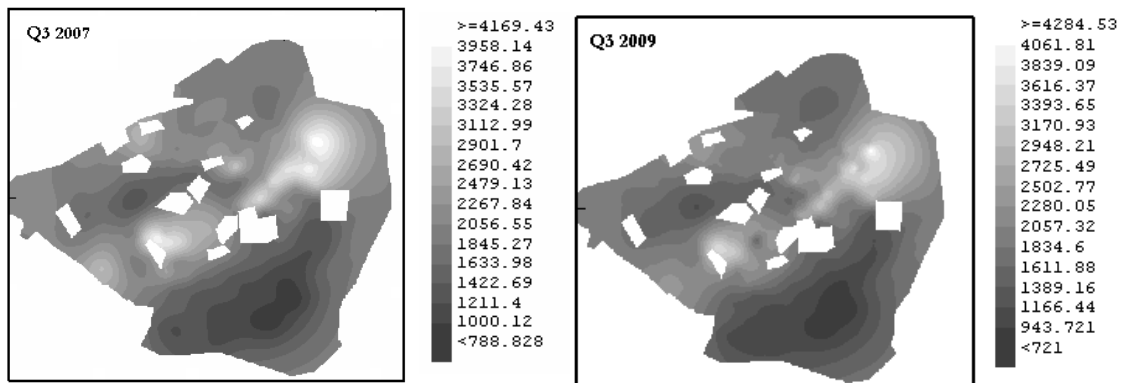
FIGURE 3: Cokriging valuation of commercial property prices (€/m 2 ). Maps corresponding to Q3 2007 and Q3 2009.
