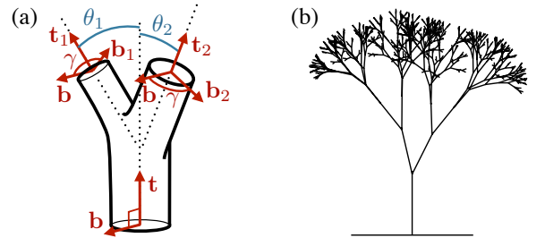
FIG. 2. Numerical tree model: (a) Sketch of the angles and unit vectors at a branching node; (b) Example of tree skeleton for \theta_1 = -15^\circ , \theta_2 = 30^\circ , \gamma = 120^\circ , r_1 = r_2 = 0.75 , p = 1 , K = 10 , D = 2.41 [as given by (9)].
