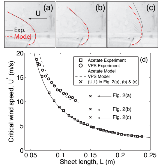
FIG. 2: (a,b,c) Photographs of a single acetate sheet (solid lines), with L = 15.0 \text{ cm} , W = 2.9 \text{ cm} , \rho_p h W = 0.114 \text{ g/cm} , and BW = 2.4 \times 10^{-4} \text{ Nm}^2 , superimposed with predicted shape (dashed lines). Flow speeds were (a) 11.1, (b) 8.5, and (c) 6.8 m/s. For all static shape calculations, we use a spatial resolution of 1000. (d) Experimental and predicted (with C_d = 1.76 ) critical wind speed versus length for two materials: acetate strip with W = 3.0 \text{ cm} , \rho_p h W = 0.118 \text{ g/cm} , and BW = 2.6 \times 10^{-4} \text{ Nm}^2 ; vinylpolysiloxane (VPS) strip with W = 2.2 \text{ cm} , \rho_p h W = 2.04 \text{ g/cm} , and BW = 2.3 \times 10^{-4} \text{ Nm}^2 , with paper on its front surface. Also shown (x) are parameter values for the photographs in (a), (b), and (c).
