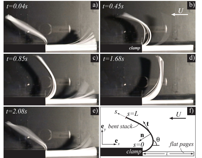
FIG. 1: (a-e) Representative photographs of the clapping book at selected times during a single period. (f) Schematic diagram of the system.
