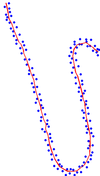
Figure 6: Principal curve fitted with the LS algorithm for the hairpin data.
