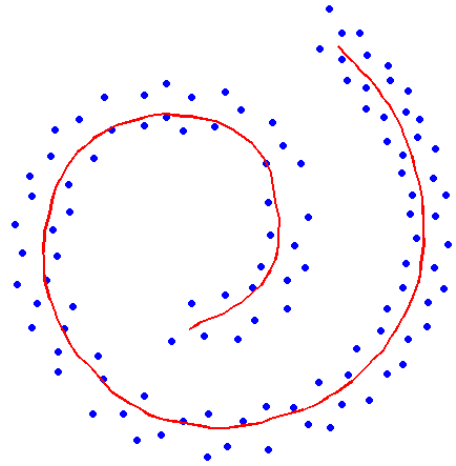
Figure 7: Principal curve fitted with the LS algorithm for the Labyrinth data.
