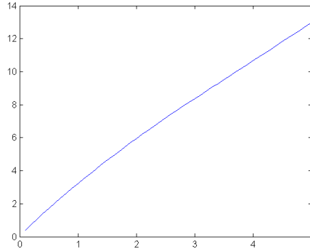
Figure 9: Function \frac{\varphi_\ell}{\kappa\sqrt{nd}} for d = 2 , \ell = 6 and \lambda = 3 .
