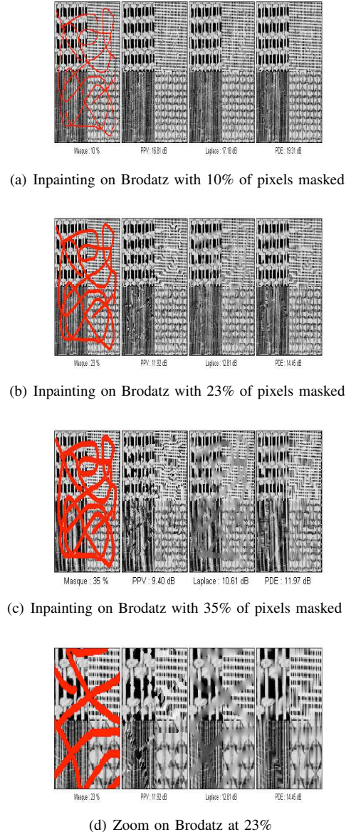
Fig. 1. Illustration of image inpainting using PDE-interpolator: Visual comparison of PDE-interpolator, kNN and Laplace methods.
