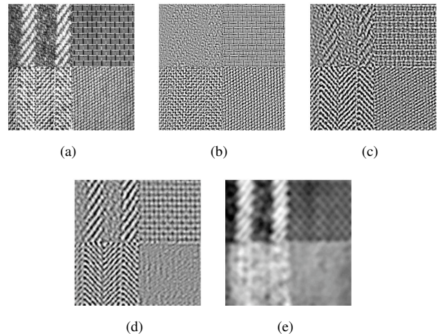
Fig. 10. Illustration of PDE-Based BEMD texture on 'Brodatz' image. (a) Original image. (b - c and d) details with successive IMFs from PDE-BEMD. (e) the residu of the EMD.
