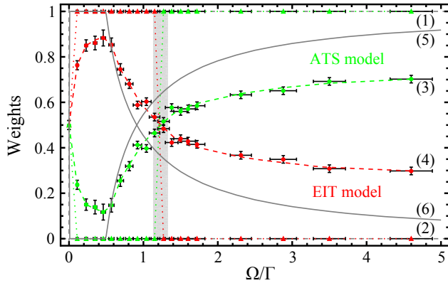
FIG. 3: (color online). Experimental Akaike weights w_j as a function of the Rabi frequency \Omega for ATS model (green triangles, curve (1)) and for EIT model (red triangles, curve (2)). Experimental per-point weights \bar{w}_j for ATS model (green dots, curve (3)) and for EIT model (red dots, curve (4)). The grey area indicates the EIT/ATS model transition. Error bars include the uncertainty on the coefficient \alpha and on the measured power. The solid lines give the theoretical per-point weights for a pure 3-level system (curves (5) and (6)).
