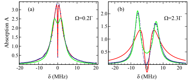
FIG. 2: (color online). Absorption profiles and model fits for two values of the control Rabi frequency \Omega . Experimental data (blue dots) are presented together with the best fits of functions A_{\text{EIT}}(C_+, C_-, \epsilon, \gamma_+, \gamma_-) (red solid lines) and A_{\text{ATS}}(C_1, C_2, \delta_1, \delta_2, \gamma_1, \gamma_2) (green solid lines). Parameters C_+ , C_- , C_1 , C_2 representing the amplitudes of the absorption curves are in dimensionless units, while the parameters \epsilon , \gamma_+ , \gamma_- and \delta_1 , \delta_2 , \gamma_1 , \gamma_2 representing detunings and widths are in MHz. (a) \Omega = 0.2\Gamma . In this case A_{\text{EIT}}(3.52, 3.14, 1.45 \times 10^{-2}, 5.71, 0.239) fits the experimental data much better than A_{\text{ATS}}(2.01, 2.04, 1.84, 1.84, 4.14, 4.08) . (b) \Omega = 2.3\Gamma . Here A_{\text{ATS}}(2.05, 1.64, 5.86, 5.67, 3.94, 4.68) fits the data better than A_{\text{EIT}}(1.59 \times 10^5, 1.59 \times 10^5, 1.45 \times 10^{-7}, 8.17, 8.17) .
