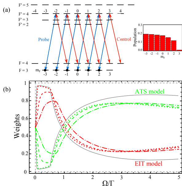
FIG. 4: (color online). Theoretical simulations with Zeeman sublevels and Doppler broadening. (a) Level scheme for the Cs D_2 line and the six three-level transitions involving Zeeman sublevels; inset: population distribution. (b) Per-point weights for a three-level system (grey solid lines), for a system involving Zeeman sublevels (dotted lines), for a system involving Zeeman sublevels and residual Doppler broadenings \Gamma_D/2\pi = 0.6 MHz (dashed lines) and \Gamma_D = 1.3/2\pi MHz (dash-dotted lines).
