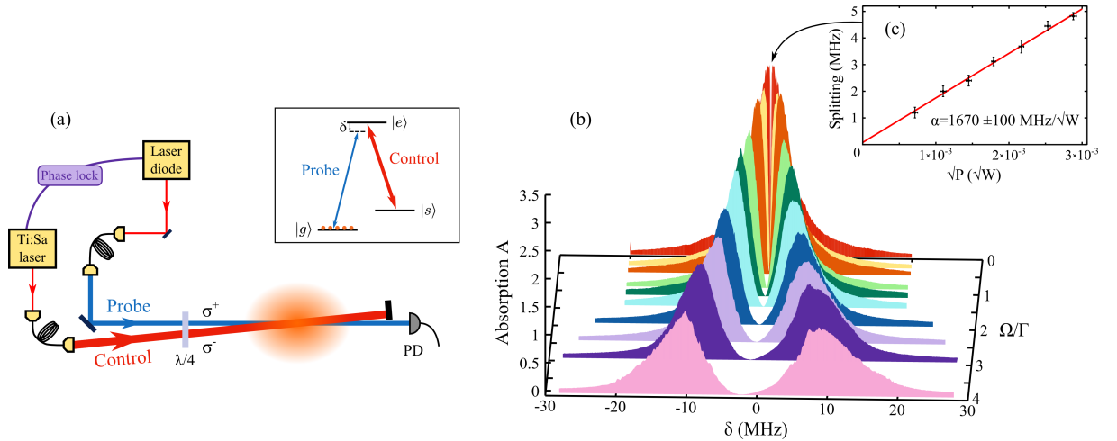
FIG. 1: (color online). Absorption in a \Lambda -type system. (a) Experimental setup: a weak probe beam and a control beam travel through a cloud of cold cesium atoms. Atoms are initially in the ground state |g\rangle . The probe field is close to the |g\rangle \rightarrow |e\rangle transition (detuning \delta ) while the control field drives the |s\rangle \rightarrow |e\rangle transition on resonance; PD : high-gain photodiode. (b) Absorption profiles are displayed as a function of the detuning \delta for a control Rabi frequency \Omega between 0.1\Gamma and 4\Gamma , where \Gamma is the natural linewidth. (c) Experimental splitting as a function of \sqrt{P} , where P is the measured control power, fitted by a linear function.
