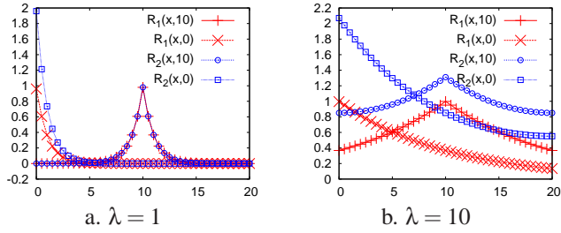
Figure 2. AUTOCORRELATION FUNCTIONS R_1(x, x_1) AND R_2(x, x_1) WITH x_1 = 0 AND 10 AS A FUNCTION OF x FOR a. \lambda = 1 AND b. \lambda = 10 .
