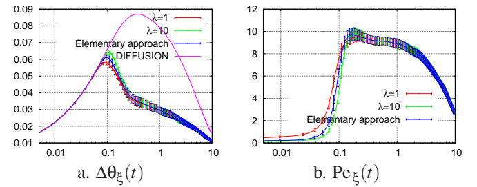
Figure 5. MEAN VALUES AND CONFIDENCE INTERVALS FOR a. \Delta\theta_\xi(t) AND b. \text{Pe}_\xi(t) .
