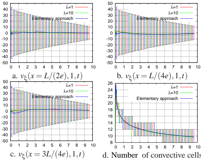
Figure 6. MEAN VALUES AND CONFIDENCE INTERVALS FOR THREE LOCAL VELOCITIES AND THE NUMBER OF CONVECTIVE CELLS.
