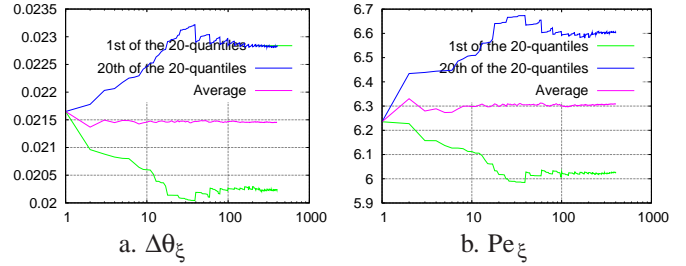
Figure 1. CONVERGENCE FOR THE ELEMENTARY APPROACH OF \langle \widehat{X}_\xi \rangle^{[i]} , \widehat{V}_1^{[i]} , AND \widehat{V}_{20}^{[i]} AS A FUNCTION OF THE NUMBER OF MONTE CARLO RUNS ( i ) FOR a. \Delta\theta_\xi AND b. Pe_\xi .
