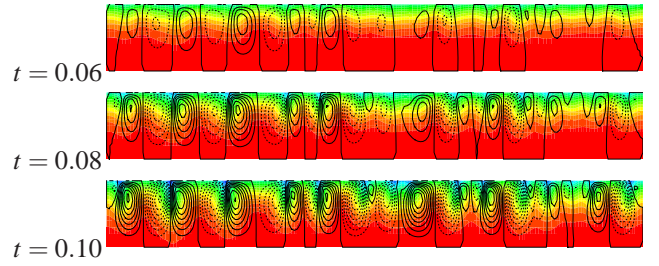
Figure 4. ISOTHERMS AND STREAMLINES AT 3 INSTANTS.
