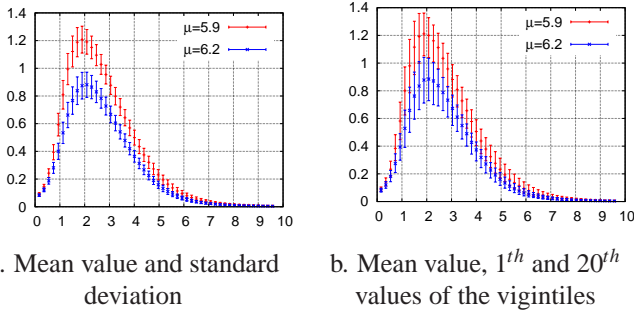
Figure 7. Pe_{\xi}(t) FOR \mu = 5.9 \text{ mPa} \cdot \text{s} AND \mu = 6.2 \text{ mPa} \cdot \text{s} .
