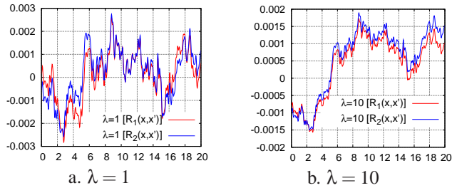
Figure 3. INITIAL THERMAL DISTURBANCES BASED ON R_1(x, x') AND R_2(x, x') AS A FUNCTION OF x FOR a. \lambda = 1 AND b. \lambda = 10 .
