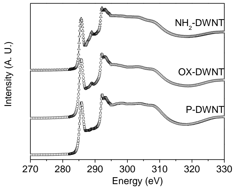
Fig. 2.C K-edge NEXAFS spectra of P-DWCNT, OX-DWCNT and \text{NH}_2\text{-DWCNT} samples.
