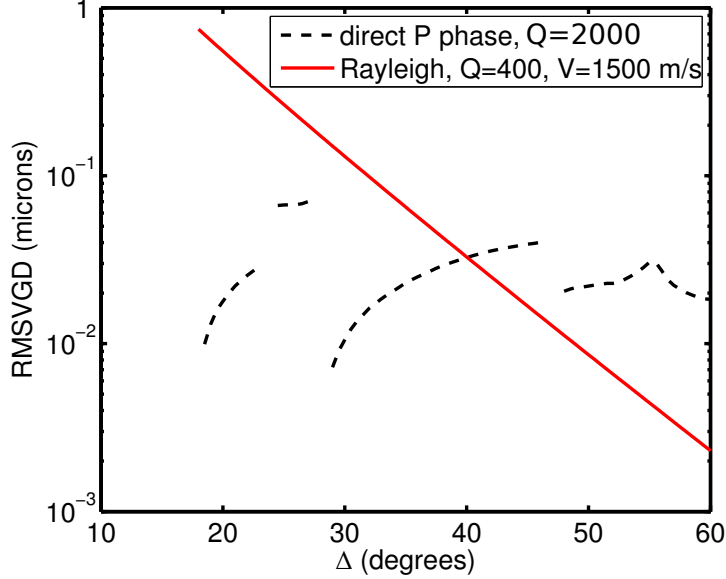
FIGURE 14. Estimates of the rms vertical ground displacement associated to Rayleigh or P waves, as a function of the epicentric angle \Delta , for a source of intensity \int F_{p2,surf}(\mathbf{K} = 0, f)df = 4.2 \times 10^4 hPa 2 m 2 over a 330 by 330 km square, assuming an attenuation factor Q = 2000 for the P waves (Pasyanos et al. 2009), with travel times given by the ak135 reference Earth model (Snoke 2009).
