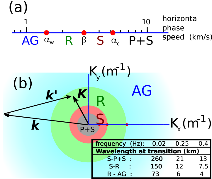
FIGURE 1. (a) Typical distribution of speeds: \alpha_w is for sound waves in the ocean, \beta and \alpha_c are shear and compression speeds in the upper crust. These velocities separate the horizontal phase speeds in four domains. From slow to fast, these are the acoustic-gravity (AG) domain, the Rayleigh (R) wave domain, and two body wave domains ( S only, and P and S together) (b) For any fixed frequency, the four domains correspond to 4 concentric regions in the wavenumber plane. For three selected frequencies in the infragravity, dominant and high frequency ranges of the forcing wave field, the limiting wavelengths between the four domains are indicated. One example of interaction (black vectors) is shown with two gravity wave modes that interact to generate a Rayleigh waves.
