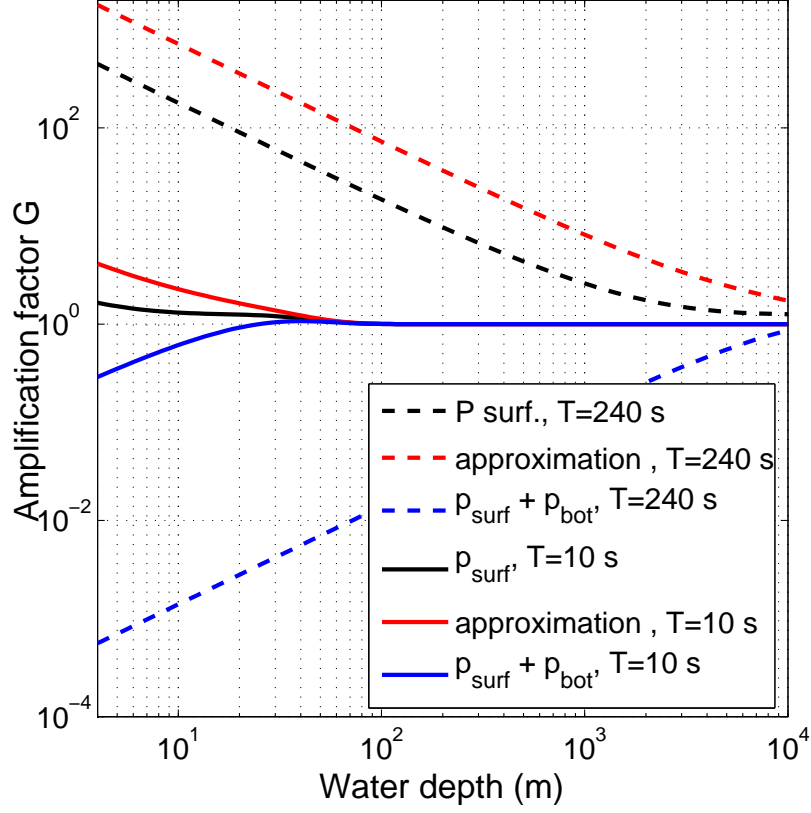
FIGURE 4. Compared to deep water, the source of seismic noise power in finite water depth is amplified by a coefficient G(kh) = \tanh^2(kh) [1 + 2kh/\sinh(2kh)] , when accounting for both the surface and bottom forcing. This is very different from the approximation that considers the surface forcing only (leading to eq. 2.25), even more so when using its deep water approximation (eq. 2.19) which gives a factor 4 difference for kh \ll 1 .
