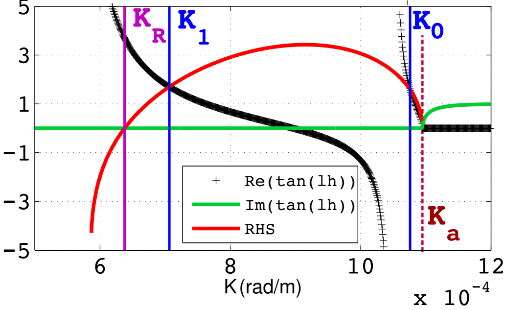
FIGURE 7. Wavenumbers of seismic and acoustic modes for a fixed frequency, which are the solutions of eq (4.24), for which the right hand side (RHS) equals the real part of \tan(lh) . Here we used h = 5000 m, \alpha_w = 1500 m/s, \beta = 3200 m/s, \rho_w = 1000 kg/m 3 and \rho_s = 2500 kg/m 3 . This graph corresponds to a seismic frequency f_s = 0.263 Hz, for which f_s h / \alpha_w = 0.88 . Here the determinant has three real roots, one acoustic mode K_a for which l = 0 (horizontal propagation) and two seismic modes K_0 et K_1 . The number of these roots increases with the frequency. One new solution appears every time 2\pi f_s becomes larger than \omega_{s,cj} defined by eq. (4.29). For reference we also give the wavenumber for which the right hand side of eq. (4.24) is zero, which is the Rayleigh wavenumber K_R in the absence of the ocean layer ( h = 0 ).
