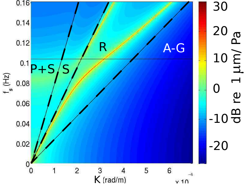
FIGURE 9. Magnitude of the transfer function G(K, f_s) illustrating the singularities along the dispersion relations of the free Rayleigh modes with wavenumbers K = K_n(f_s) . The oblique dashed lines correspond to phase speeds equal to \alpha_c , \beta , and \alpha_w , and separate the four domains body waves (P+S), mixed body and evanescent waves (S), Rayleigh waves (R) and acoustic-gravity modes (A-G).
