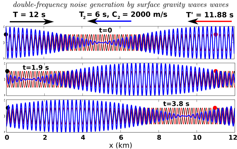
FIGURE 3. Generation of supersonic wave groups (in blue) by the superposition of two opposing deep water monochromatic wave trains of nearly equal periods T and T' . Each curve shows the surface elevation of the individual wave trains (black and red) or their combination (blue). The length of the group is 12 km, and propagates in the same direction as the wave train with the shortest wavelength. If the wave trains do not face exactly, then the group propagates in the direction of the vector \mathbf{K} = \mathbf{k} + \mathbf{k}' . The red and black dots are fixed on wave crests of each train, and move 100 times slower than the blue group.
