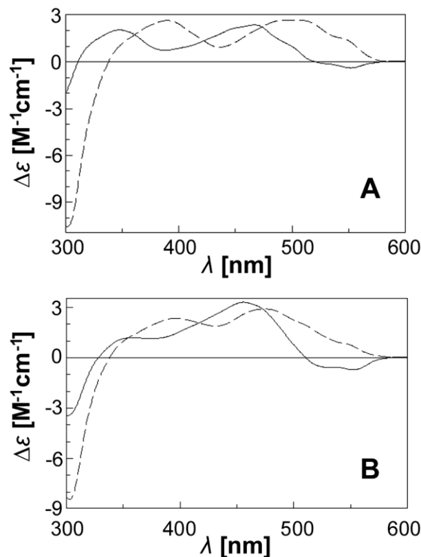
Figure S1. The circular dichroism (CD) spectra of DOX (A) and p-DOX (B) in the absence (full line) and presence (dashed line) of calf thymus DNA ( 0.27 \text{ mg mL}^{-1} ), r = 0.05 . Absorption spectra were taken in 3-cm cells at 25^\circ\text{C} in BPES buffer.
