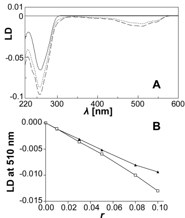
Figure S2. The linear dichroism (LD) spectra of calf thymus DNA ( 98 \mu\text{g mL}^{-1} ) incubated with DOX (A) or p-DOX (B) r = 0.1 at 37^\circ\text{C} in BPES buffer. DNA in absence (full line) and presence of DOX (dashed line) or p-DOX (dotted line). (B) The effect of increasing r on intensity of LD at 510 nm of DNA incubated with DOX (empty square) and p-DOX (full triangle).
