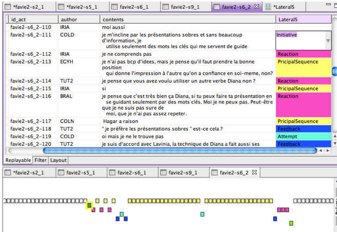
Figure 1. A screenshot of TATIANA showing the categorization of a lateral (parallel) sequence
