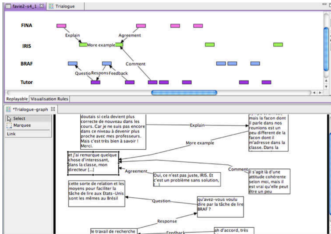
Figure 4. Visualizing an interaction scheme in progress (dialogue and triologue in parallel)
