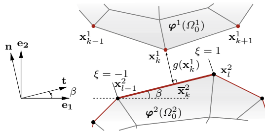
Figure 5 – Orthogonal projection of a contact node.
