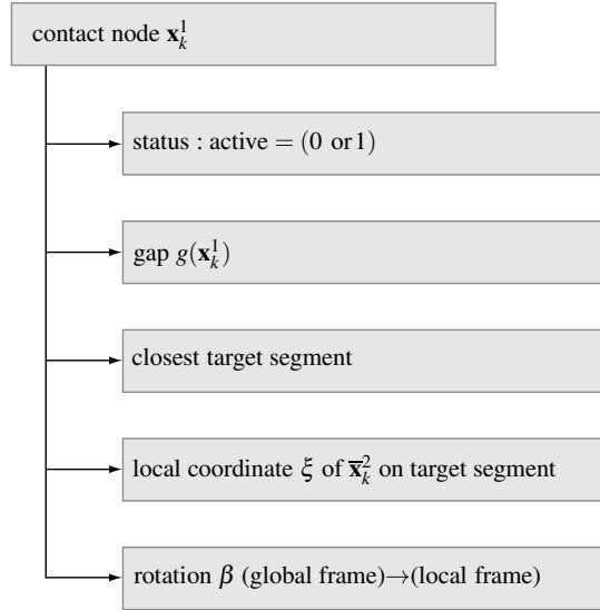
Figure 6 – Definition of a contact node.
