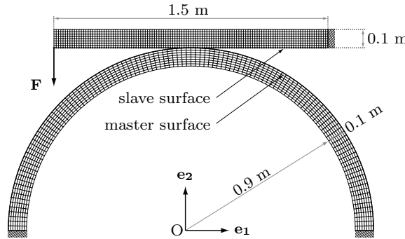
Figure 15 – Contact configuration of case 1.
