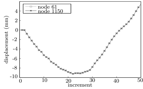
Figure 19 – Displacement of nodes 61 and 1150 along \vec{e}_2 obtained with the B-spline smoothing method.
