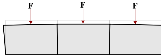
Figure 9 – Punctual forces applied on Q4 elements
