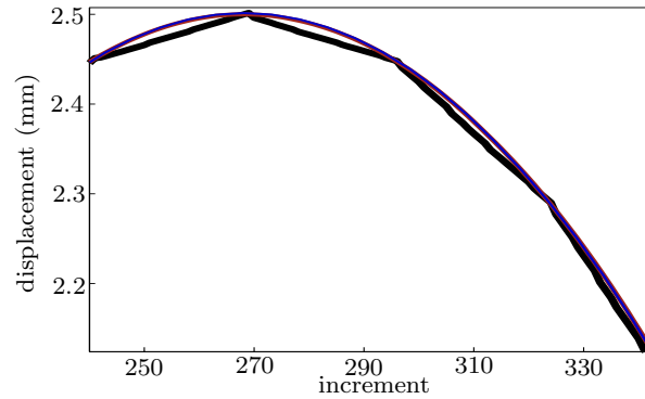
Figure 21 – Displacement of node 2179 in the \vec{e}_1 direction for linear mesh —, linear mesh with B-spline — and Hermite elements —.
