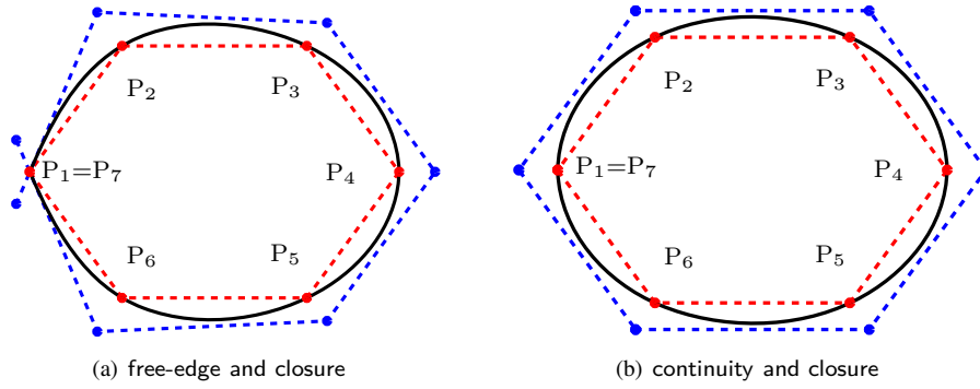
Figure 7 – two types of end condition: spline (—), data points \mathbf{P} (•) and control points \mathbf{Q} (•)
