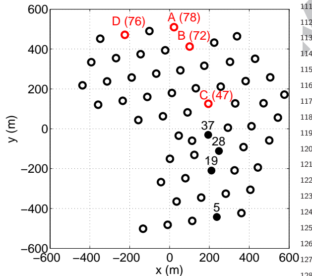
49 Fig. 1. SPATS geometry and IceCube footprint in 2009. 50 The permanently deployed SPATS hardware is indicated by 51 open circles with the string ID (ABCD) and corresponding 52 IceCube hole number. The full circles indicate the location 53 of the holes, indexed by the corresponding IceCube hole 54 number, where the pinger was deployed in the 2008-2009 55 season.
