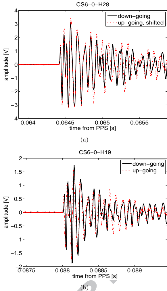
Fig. 3. Waveforms recorded by the same channel when the pinger was stopped while lowering and while raising, for two different holes at a distance of 243 m (top) and 336 m (bottom). Clock drift correction and averaging of the 180 recorded pulses have been applied. In the top plot, one of the waveforms has been shifted in time to overlap with the other one. This slight shift is due to a slight difference in the pinger depth between the two runs (see [21]).
