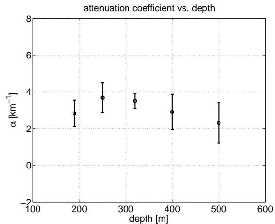
Fig. 6. Mean attenuation coefficient as a function of the depth.
