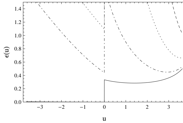
Figure 14. Adiabatic control function \epsilon as a function of u for r_0 = 4m and delays \widetilde{\Delta t}_0 = (0, 4m, 10m, \infty) [curves depicted respectively as (- - - -, ·····, - · - ·, —)]. We use 2m = 1 units and u_0 = 0 .
