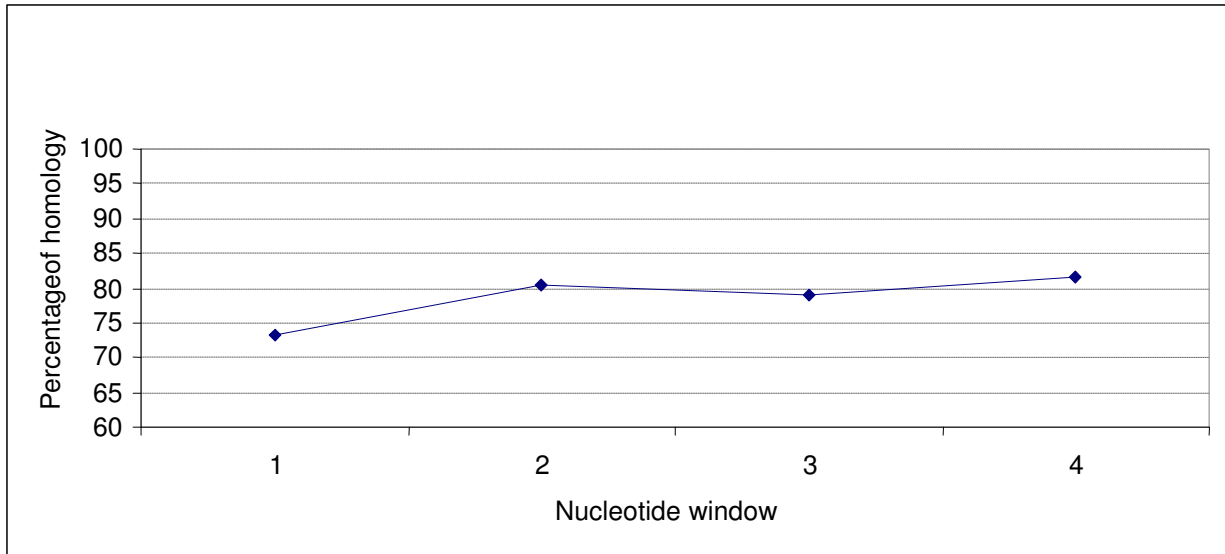
Figure 5. Average level of homology between four strains of IBV in four different windows of 400 nucleotides of nucleotides 1-1600 of the S1 region on the S gene of different genotypes/serotypes (Adznaret al., 1997).
