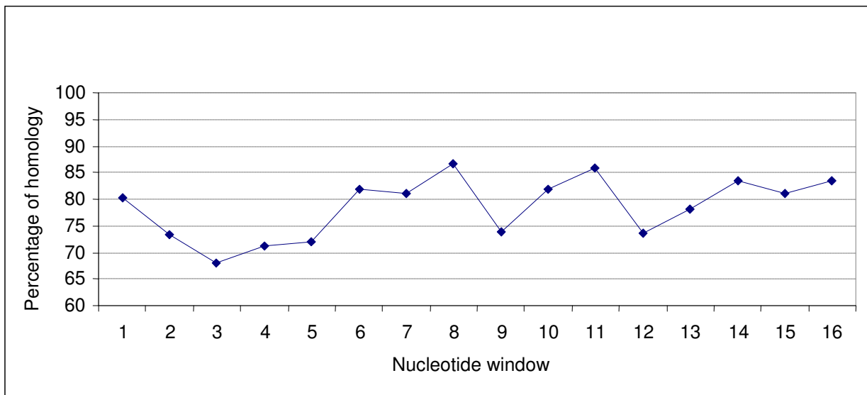
Figure 4. Average level of homology between four strains of IBV in 16 different windows of 100 nucleotides of nucleotides 1-1600 of the S1 region on the S gene of different genotypes/serotypes (Adznar et al., 1997).
