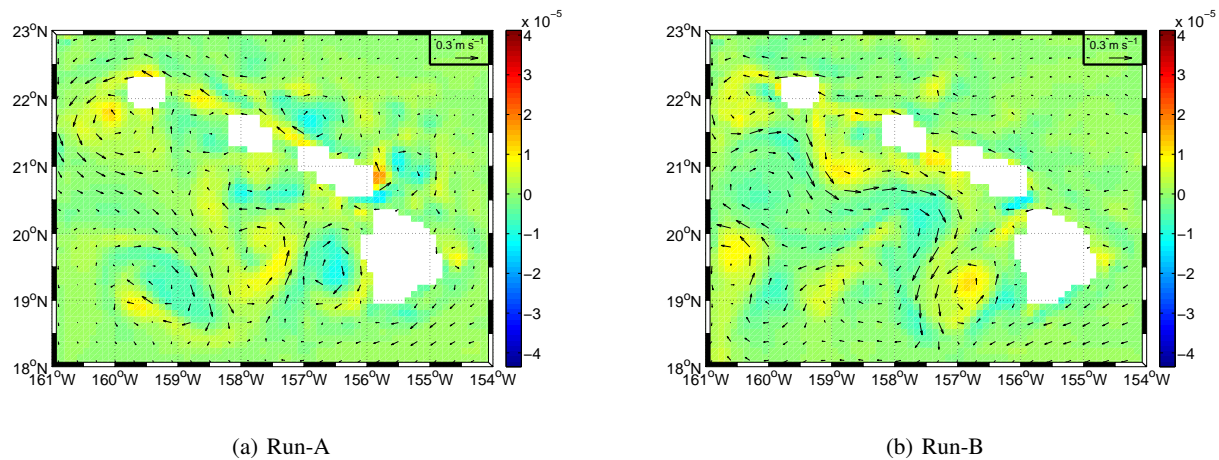
Fig. 4. Relative vorticity field with velocity vectors at 10-m depth on 22 August for Run-A (left) and Run-B (right).
