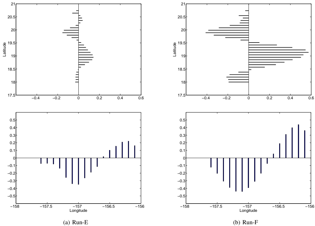
Fig. 12. East-west horizontal velocity [ \text{m s}^{-1} ] component at 40-m depth vector across a north-south transect (top) and north-south horizontal velocity component across a east-west transect (bottom) of the eddy C5-E (Run-E, 13 April, left) and of the eddy C1-F (Run-F, 28 March, right).
