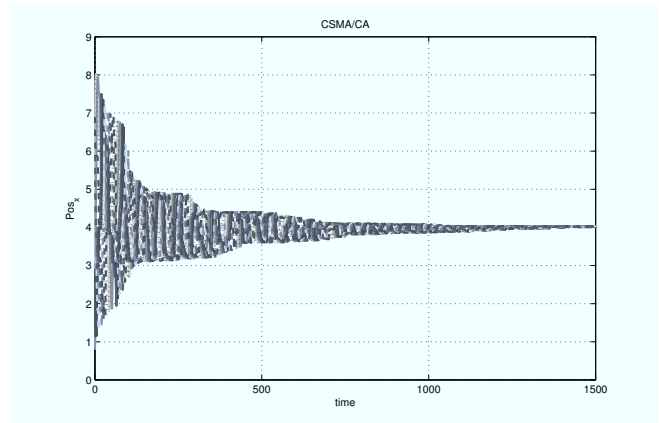
Fig. 9. Multi-agent consensus using IEEE 802.11
