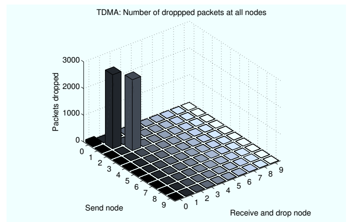
Fig. 3. Packet drop using TDMA. Simulation time = 60 sec.
