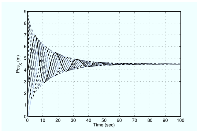
Fig. 6. Multiple quadrotor consensus with \tau_{ji} = \tau_{kj}
