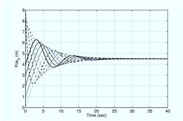
Fig. 2. Multiple quadrotor consensus using perfect communication
