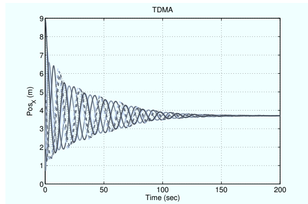
Fig. 10. Multi-agent consensus using TDMA
