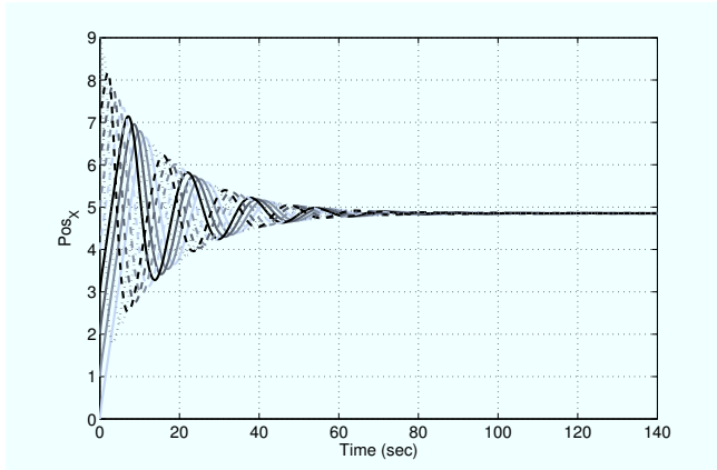
Fig. 7. Multiple quadrotor with \tau_{ji} \neq \tau_{kj}
