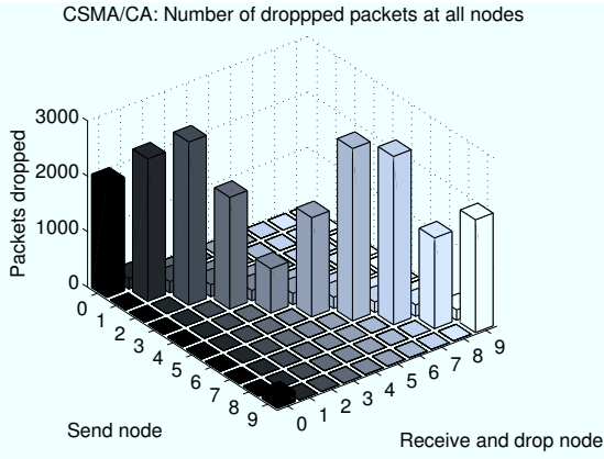
Fig. 4. Packet drop using CSMA/CA. Simulation time = 60 sec.
