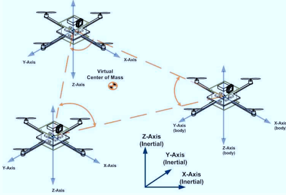
Fig. 1. Quadrotor platoon
