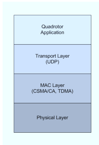
Fig. 8. Multiple quadrotor wireless network stack
