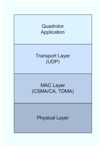
Fig. 8. Multiple quadrotor wireless network stack
