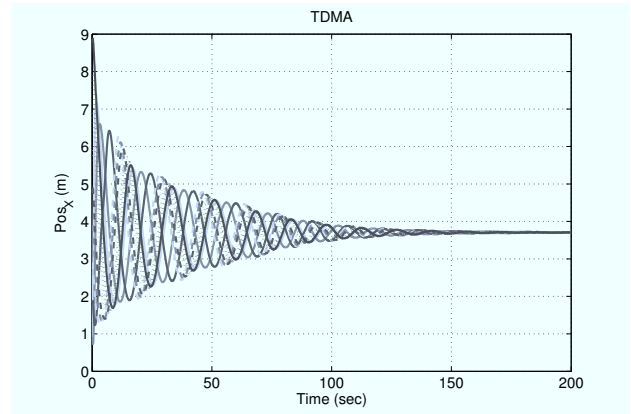
Fig. 10. Multi-agent consensus using TDMA
