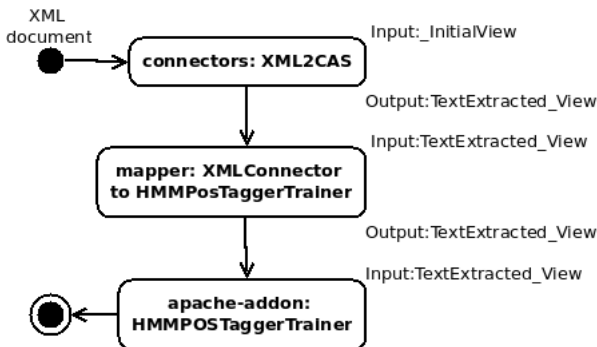
Figure 2: Mapping annotations: from the FTB to the HMMPOSTaggerTrainer.
