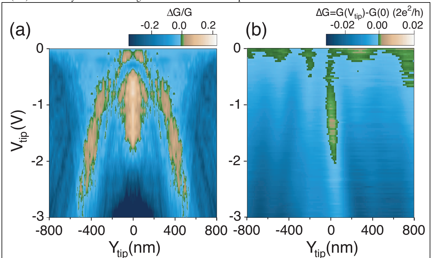
FIGURE 3 (a) Conductance variation map as a function of V_{tip} and Y_{tip} in the middle of a Braess-paradox device ( X_{tip} = 0 ). The corral length and width are 0.8 \mu\text{m} and 1.6 \mu\text{m} . The width of the openings, lateral arms, and central branch are 340 nm, 140 nm, and 160 nm, respectively. V_{DS} = 1 \text{ mV} . \lambda_F = 47 \text{ nm} . (b) A zoom on the experimental image of Fig. 2(c) over the same voltage-position window as in (a). The data have been centered on point C to account for the misfit of 270 nm between topographic and electrostatic images discussed in the text.
