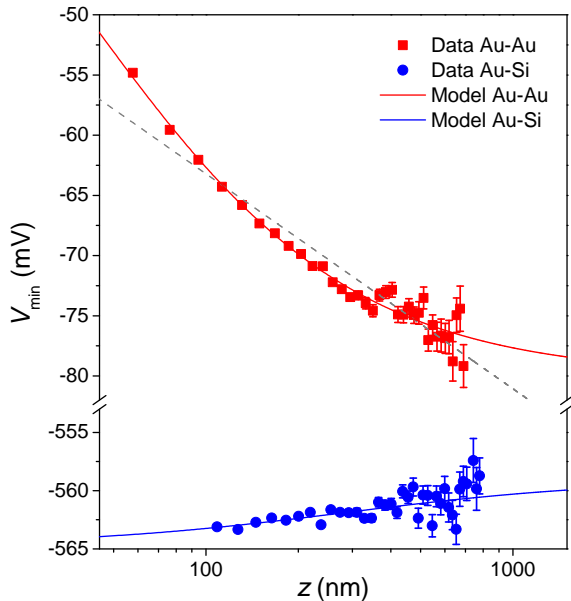
FIG. 6: Evolution with distance of the potential V_{\min} applied at 4.2 K on the sample surface to minimize the electrostatic force on the Au-Au and Au-Si sphere-plane cavities. Experimental data are fitted by the electrostatic model Eq. (5) (solid lines) and by a logarithmic function (dashed line).
