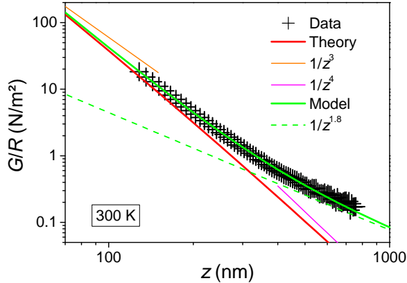
FIG. 3: Reduced force gradient at V_{\min} versus distance between two gold surfaces in sphere-plane geometry (measured at 300 K). Experimental data are compared with the theoretical prediction of the real Casimir force and with a model containing an additional long-range contribution scaling like 1/z^{1.8} .
