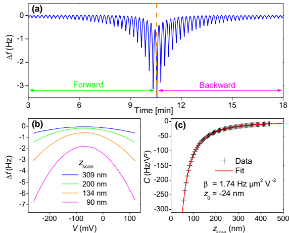
FIG. 2: (a) Frequency shift \Delta f of the cantilever resonance as a function of the time elapsed during a forward (left) and backward (right) scan of the sample toward the sphere fixed on the cantilever. Forward and backward scans are not perfectly symmetric because of the scanner hysteresis. (b) Examples of \Delta f(V) parabolas recorded by sweeping the probe-surface bias V for different scanner positions z_{\text{scan}} . (c) Fit of the parabola curvatures C versus scanner position z_{\text{scan}} used to obtain the force calibration factor \beta and the position z_0 of the contact.
