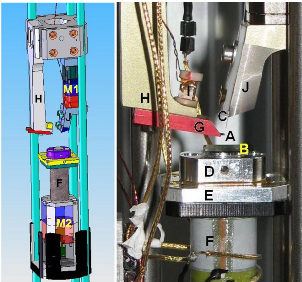
FIG. 1: Drawing and photograph of the microscope head at the bottom part of the cage structure. The functional parts of the microscope, labeled by capital letters, are described in the text.
