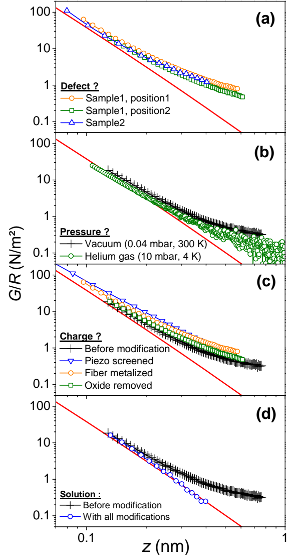
FIG. 4: Analysis of the long-range residual force at V_{\min} showing the reduced force gradient G/R between two gold surfaces measured at 300 K in vacuum: (a) at two positions located 1 mm apart and on a different sample with the same probe; (b) at different temperatures and gas pressures; (c) after a single change in the environment, either Faraday cages around piezoelectric elements, or gold coating of the optical fiber, or removal of the oxide layer covering the anodized chip holder; (d) with the three above modifications implemented together.
