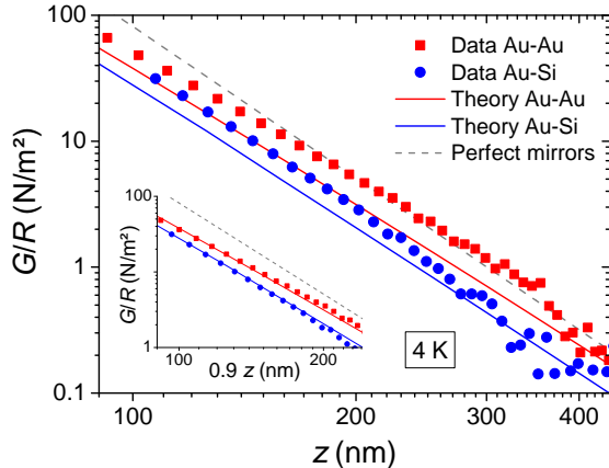
FIG. 7: Reduced Casimir force gradient G/R versus distance z measured at 4.2 K between a gold sphere and a gold surface or a doped silicon surface. Data are compared with theoretical predictions for Au-Au and Au-Si cavities. The case of perfect mirrors is shown by a dashed line. Inset: same data G/R plotted for distances artificially reduced by a factor 0.9 to show that a systematic error in the calibration might be the origin of the discrepancy between experiment and theory.
