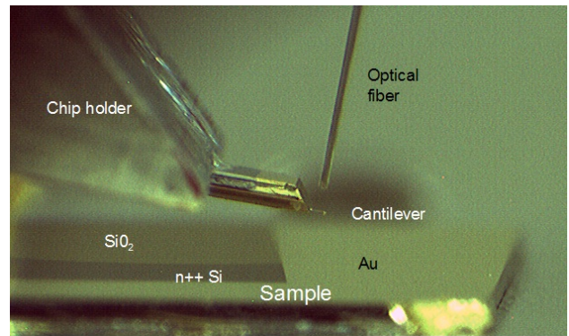
FIG. 5: Photograph showing the force probe, the optical fiber, and the sample made of a highly doped silicon substrate partly covered by 150 nm of gold (a third region is covered with a layer of silicon dioxide).
