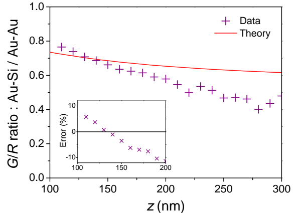
FIG. 8: Ratio between the force gradients measured for Au-Si and Au-Au cavities, compared with the theoretical prediction. Inset: relative error between experiment and theory.
