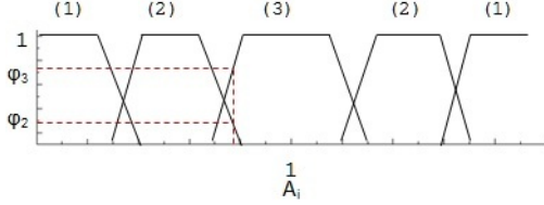
Fig. 1. Membership functions
