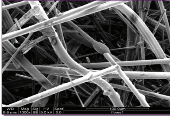
FIGURE 1 Scanning Electron Microscopy of L1.
