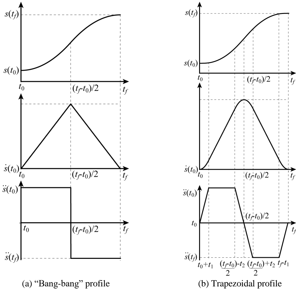
Figure 1. Motion profiles used for the shaking force minimization.
