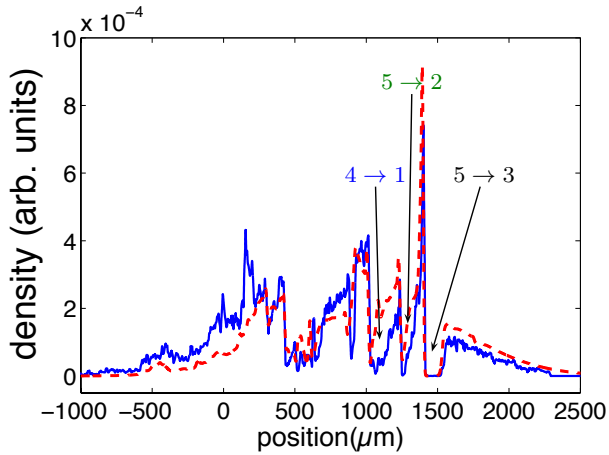
FIG. 5: Dashed line: Result of the resolution of the 1D Schrödinger equation. Solid line, result of the semiclassical simulation with random Landau-Zener transition. The arrows indicate the main processes for three depletion lines. The wave packet has a mean velocity \bar{v} = 10 mm/s and a velocity dispersion \Delta v = 6 mm/s.
