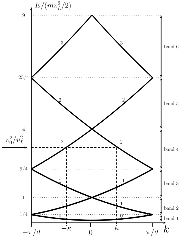
FIG. 2: The band diagram is constructed by the superposition of parabolic energy spectra centered around all reciprocal points E_n(k) = \hbar^2(k - nk_L)^2/2m . For each band we have indicated the index n of the parabola from which the corresponding branches have been constructed.
