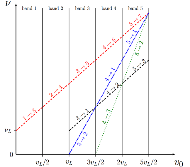
FIG. 3: (color online) Schematics of the different depletion lines observed in Fig. 1 of the article along with the numbers of the bands involved in the transition driven by the frequency of the amplitude modulation. With the experimental parameters, v_L \simeq 7.1 mm/s.
