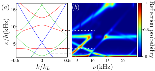
FIG. 4: (color online) (a) Floquet-Bloch band diagram for a square-envelope lattice (depth U_0 = 2E_L ) and modulation frequency \nu = 11 kHz. Band color code: green -0.5 < \langle n_F \rangle < 0.5 , red \langle n_F \rangle > 0.5 and blue \langle n_F \rangle < -0.5 where n_F is the Floquet excitation number. (b) Probability of reflection obtained from a numerical simulation of a 1D wavepacket with an incident velocity dispersion \Delta v = 0.2 mm/s impinging on time amplitude-modulated lattice with a finite square-envelope (length=80 d , U_0 = 2E_L , \eta = 30\% ) as a function of the incident energy and \nu . The horizontal white dashed line shows the case \nu = 11 kHz that corresponds to the diagram (a). The horizontal dashed (dotted) lines denotes open gap (degenerate) anticrossings. Only open gap anticrossings yield reflection.
