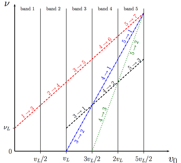
FIG. 3: (color online) Schematics of the different depletion lines observed in Fig. 1 of the article along with the numbers of the bands involved in the transition driven by the frequency of the amplitude modulation. With the experimental parameters, v_L \simeq 7.1 mm/s.
