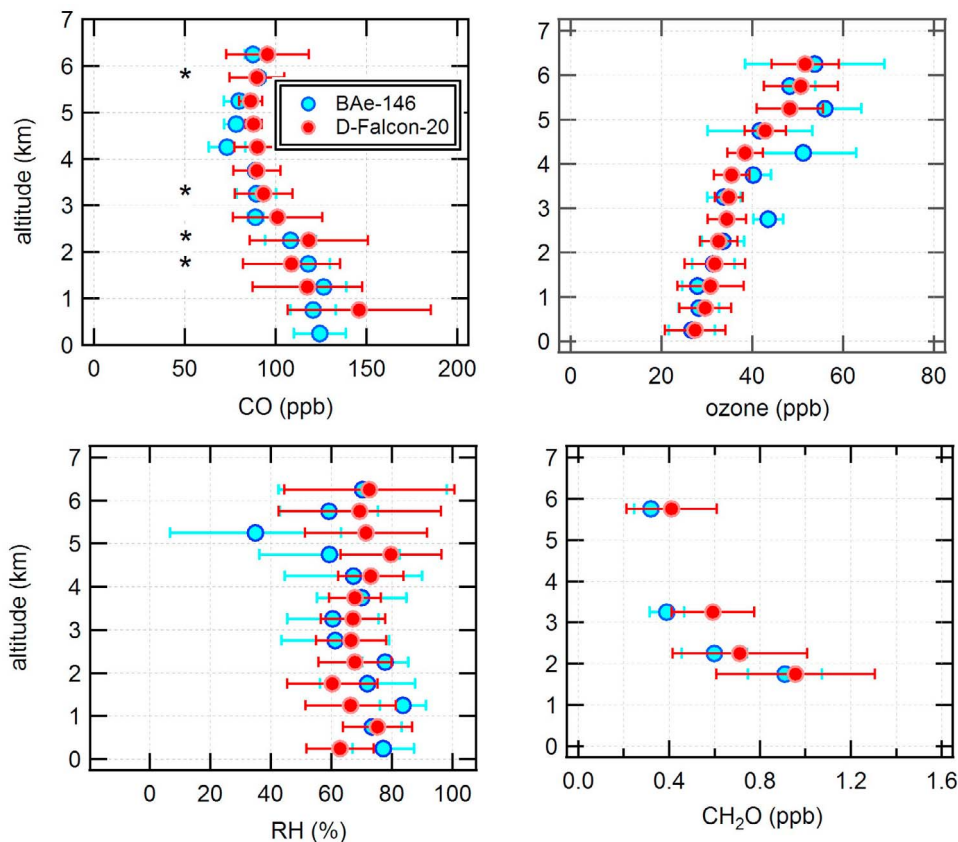
Figure 2. Comparison of the 3 physico-chemical tracers (CO, ozone and relative humidity, RH) and CH 2 O from the BAe-146 and D-Falcon20 aircraft in zone 1. The stars mark the altitude bins where physico-chemical tracers are statistically comparable.
