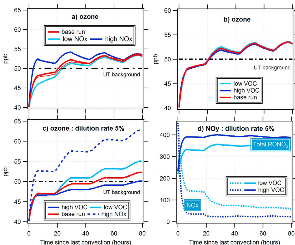
Figure 9. Time dependent simulation of ozone and \text{NO}_y evolution in MCS outflow over West Africa under different scenarios regarding (a) \text{NO}_x , (b) VOC, (c) dilution rate and (d) VOC at a low dilution rate of 5%.
