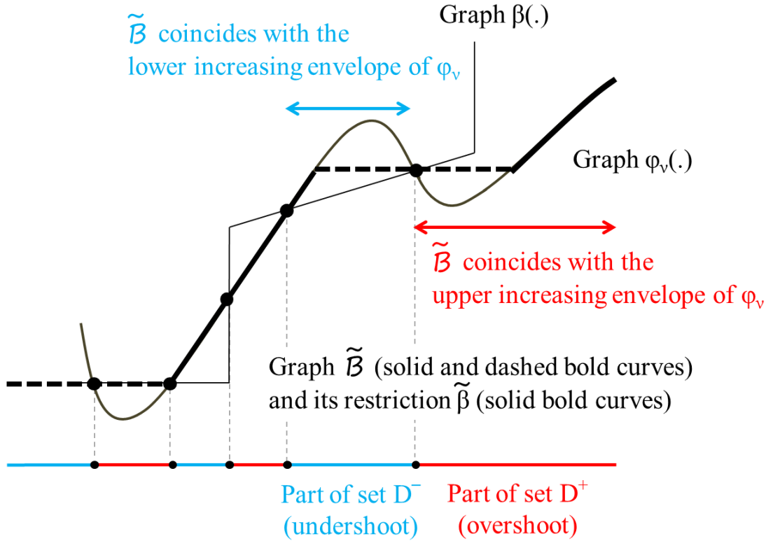
FIGURE 1. Example of construction of the projected graph \tilde{\beta}
