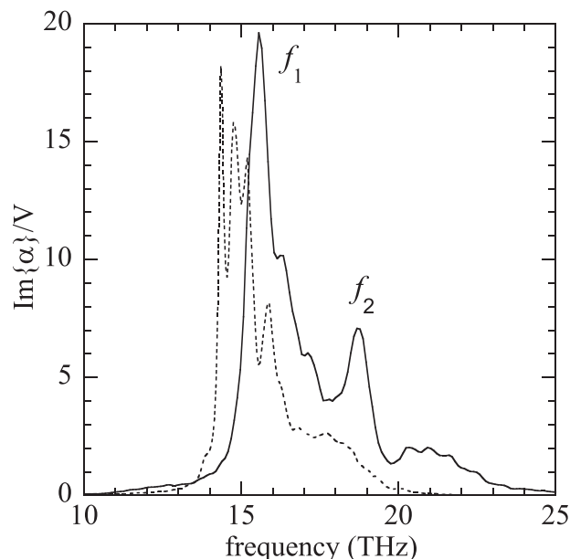
FIG. 2. Imaginary part of the NP polarisability derived from MD simulation (solid line, 4.2 nm size) and compared to finite elements method (FEM) for Maxwell equations in the electrostatic approximation (dashed line, 4.2 nm size). The three FEM peaks around 15 THz are due to the mesh discontinuities at the cube edges. A single peak is observed when smoothing the edges.
