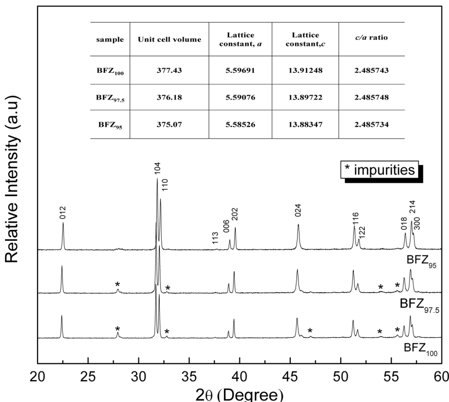
FIG. 1. X-ray diffraction patterns of \text{Bi}_x\text{Fe}_{0.9}\text{Zr}_{0.1}\text{O}_3 ( x = 1, 0.975, 0.95 ) ceramics (table inset sums up cell parameters).
