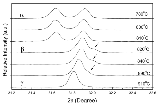
FIG. 4. HTXRD patterns of \text{BFZ}_{95} ceramic at selected temperatures, focusing on the resolution of the pseudocubic (110)_c reflection through the \alpha \leftrightarrow \beta \leftrightarrow \gamma phase transitions.
