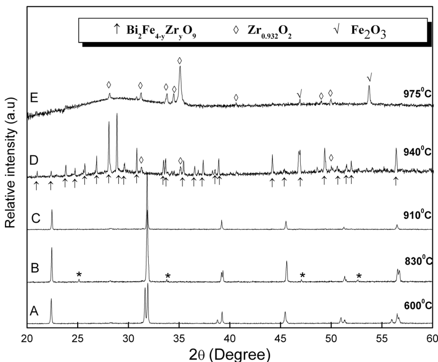
FIG. 3. X-ray diffraction patterns of \text{BFZ}_{95} ceramic recorded under different temperatures (asterisk: weak diffraction peaks observed in the diffraction pattern recorded at 830 °C).
