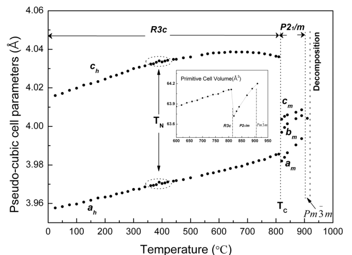
FIG. 5. Temperature-dependence evolution of the R3c, the P2 1 /m, and Pm \bar{3} m cell parameters of BFZ 95 ceramic described in a pseudocubic cell ( a_h = a_H/\sqrt{2} , c_h = c_H/\sqrt{12} ) and a_m = a_M/\sqrt{2} , b_m = b_M/2 , c_m = c_M/\sqrt{2} ).
