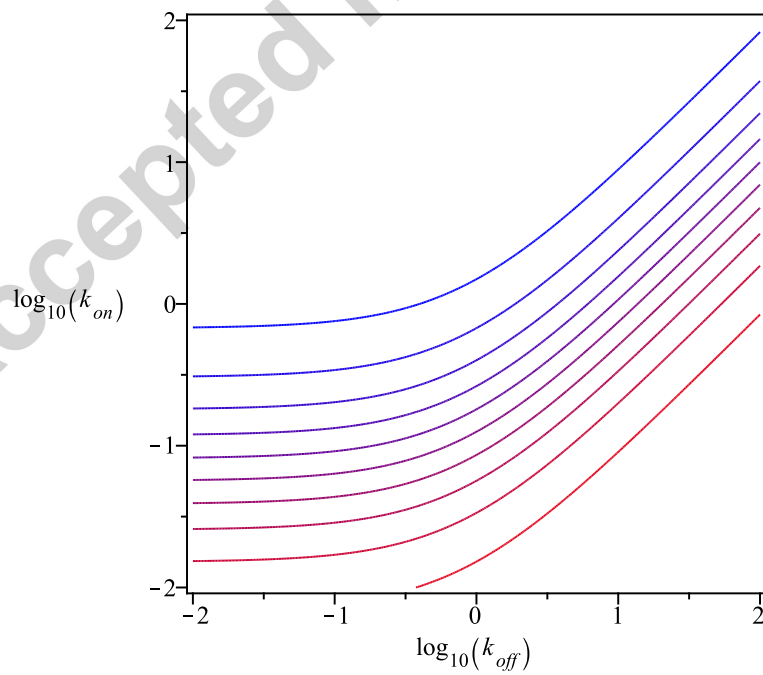
Figure 7: Contours of the surface shown in Fig. 6 for constant values of R_{\min} .
