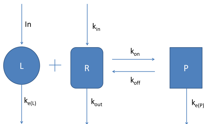
Figure 1: The TMDD reaction mechanism
