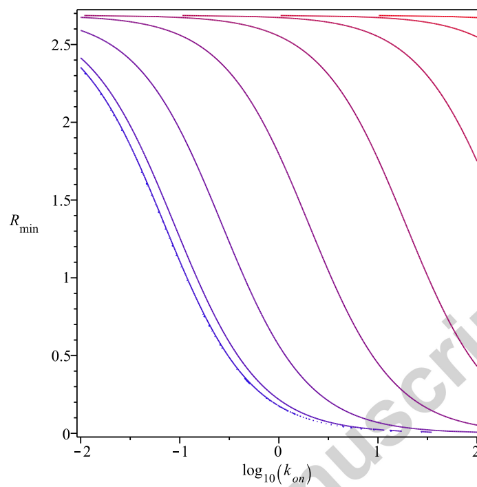
Figure 8: Contours of the surface shown in Fig. 6 for constant values of k_{off} .
