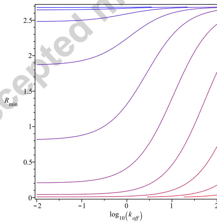
Figure 9: Contours of the surface shown in Fig. 6 for constant values of k_{on} .
