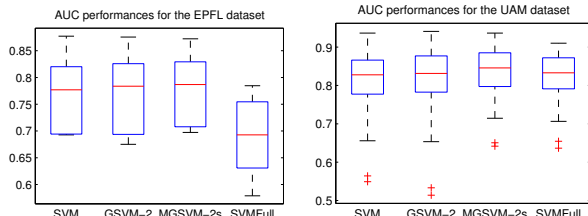
Fig. 8. AUC performances comparison with EPFL (left plot) and UAM (right plot) for 500 training examples per subject.
