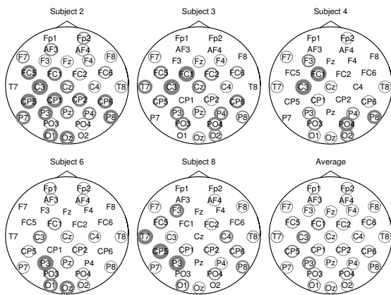
Fig. 2. Selected sensors for the EPFL dataset. The line width of the circle is proportional to the number of times the sensor is selected for different splits. No circle means that the sensor has never been selected.
