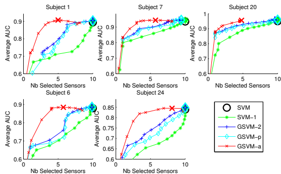
Fig. 5. Performance vs sensor selection visualisation for the UAM dataset. The large marker corresponds to the best model along the regularization path.
