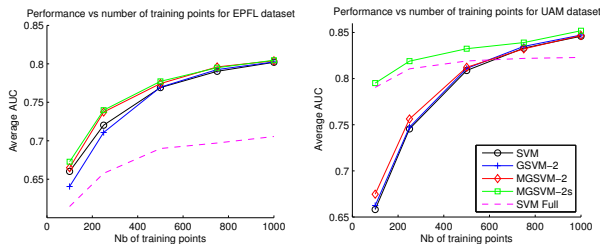
Fig. 7. Multi-task learning performances (AUC) for the EPFL (left plot) and UAM (right plot) datasets for different number of training examples per subject.
