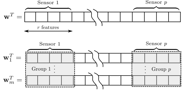
Fig. 1. Examples of feature grouping for (top) single task and (bottom) multiple task learning.
