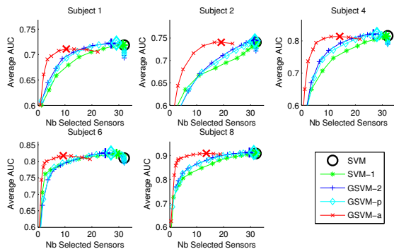
Fig. 4. Performance vs sensor selection visualisation for the EPFL dataset. The large marker corresponds to the best model along the regularization path.
