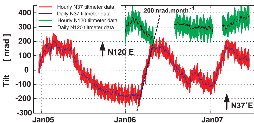
Figure 2: Two and a half years raw data. Red and blue represent decimated hourly and daily data from the N37° E instrument, orthogonal to the vein. Green and black curves represent decimated hourly and daily data from the N120° E instrument, inside the vein.
