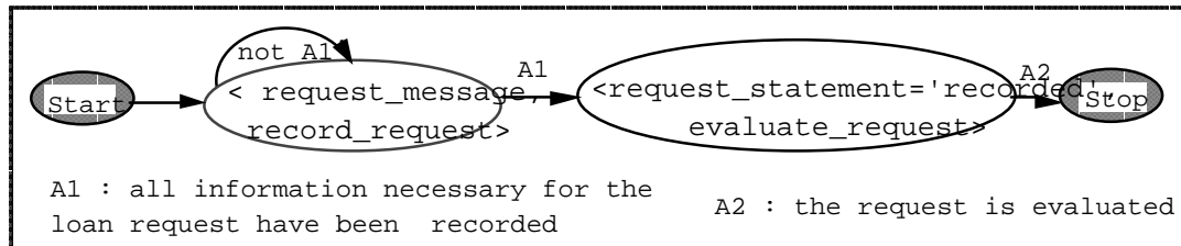
Figure 10. Example of a precedence graph
