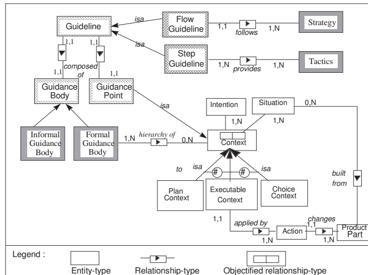
Figure 4: Guideline structure
