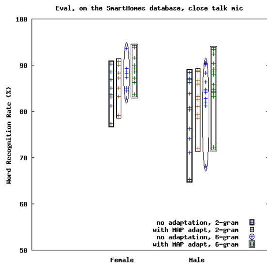
Fig. 2. Evaluations of 20 elderly speakers (lavalier microphone).
