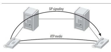
Fig. 1. SIP trapezoid architecture.
