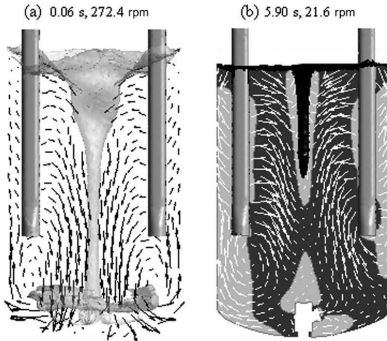
Figure 5. Radial-axial vector plots and free surface for two times from the start of the impeller slowdown; (a) black velocity vectors, free surface in light grey; (b) white velocity vectors, axial velocity contour plot with positive values in light grey and negative values in dark grey, free surface in black.
