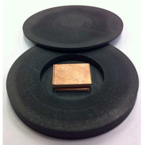
Figure 6 A photo the MPI structure in a graphite jig
