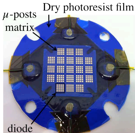
Figure 5 Photo of a wafer holder with 5\times 5 diodes and a copper foil laminated by the photoresist film, micro-posts matrix insulated and developed. The diameter of the wafer holder is 80 mm.
