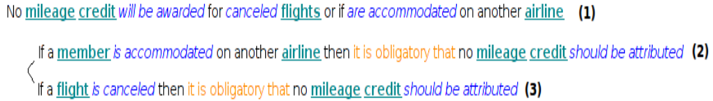
Fig. 5. SBVR translation
