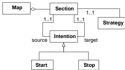
Figure 2: The map meta-model
