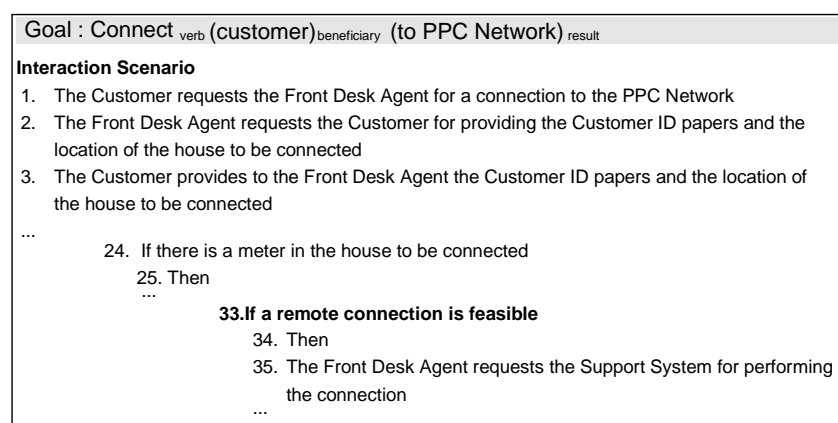
Figure 3.4 : Detailing the goal “Connect Customer to PPC network” with a scenario
