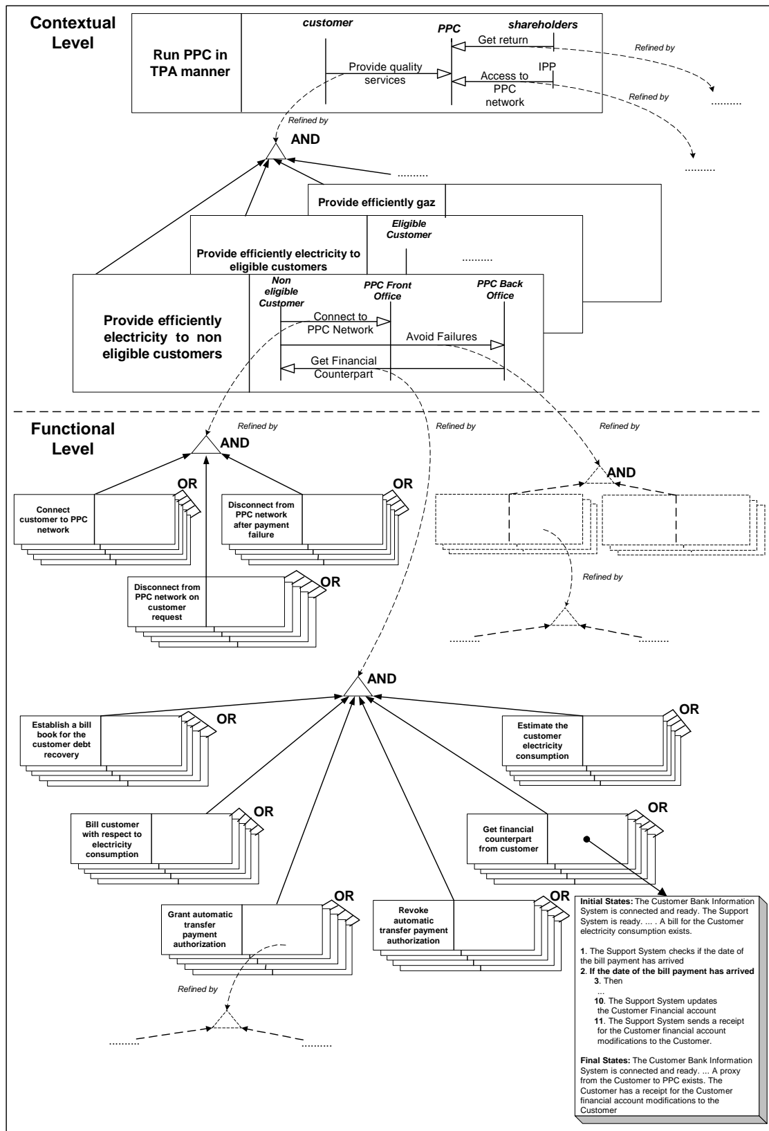
Figure 3.1 : An excerpt of the Requirement Chunks of the ELEKTRA case study
