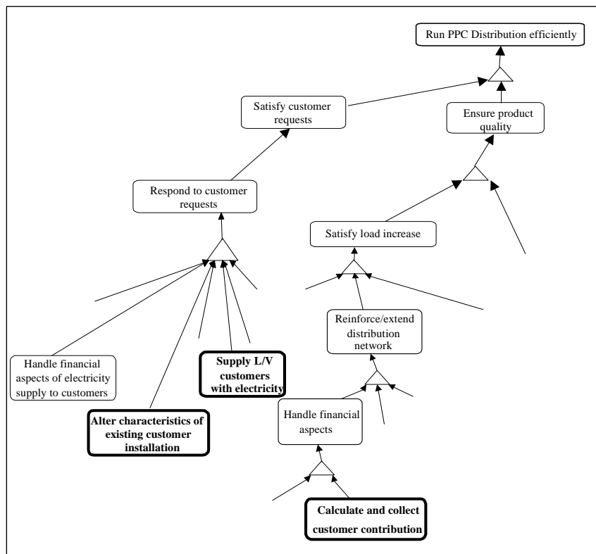
Figure A-1 : A sample of the PPC goal hierarchy showing redundancies
