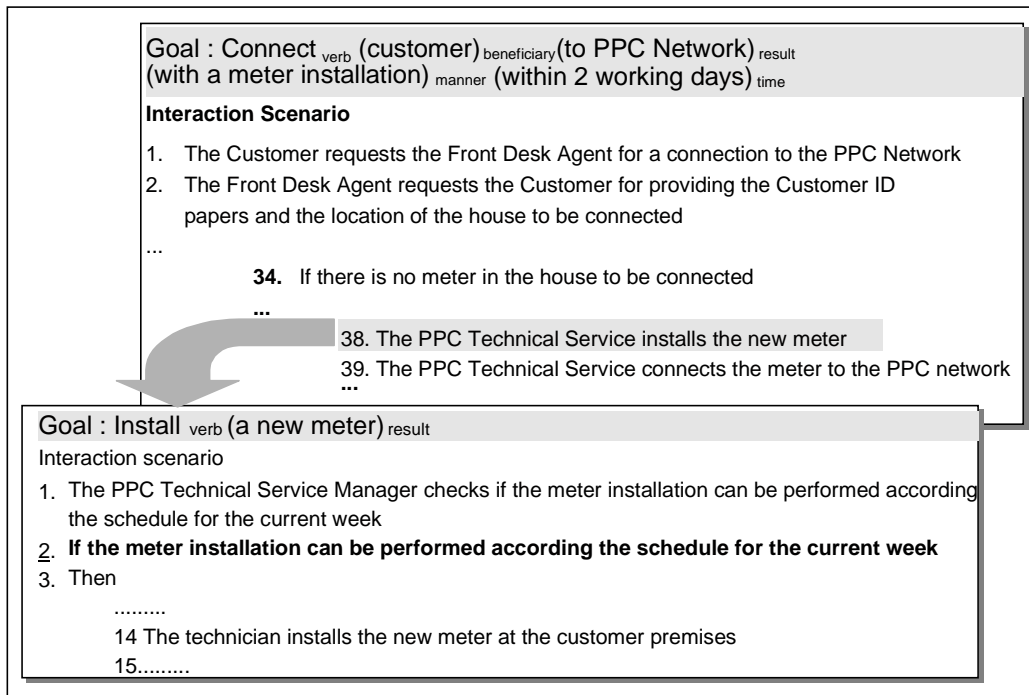
Figure 3.3 : An example of an interaction refined by a goal and its associated scenario
