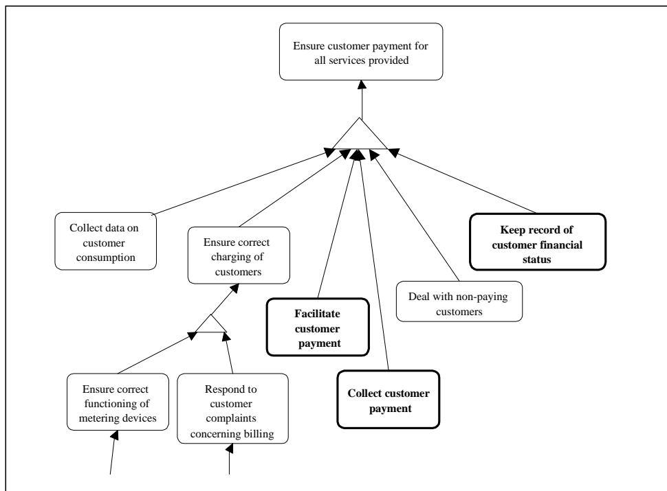
Figure A-6 : The PPC goal sub-hierarchy for “Ensure customer payment for all services provided”
