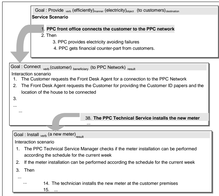
Figure 3.5 : The successive refinements of a high level goal
