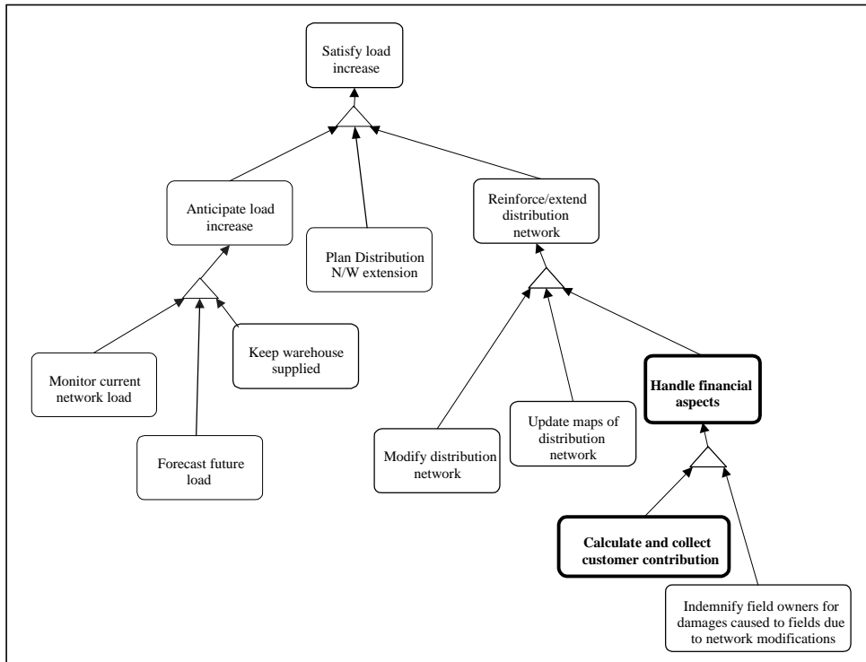
Figure A-5 : The PPC goal sub-hierarchy for “Satisfy load increase”
