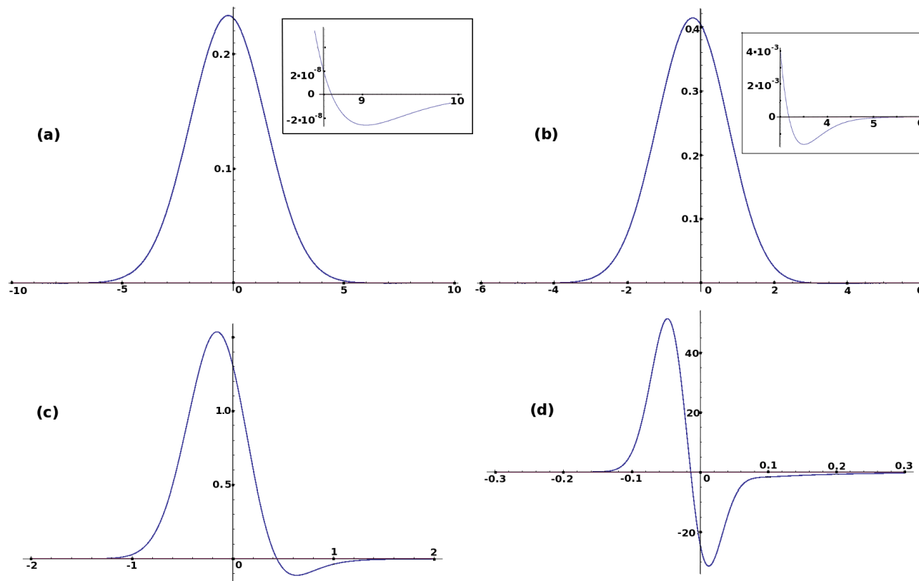
FIG. 3: Free energy "distribution function" \tilde{\mathcal{P}}_L^*(f) as it given by eq.(66) for: (a) \epsilon = 1.5 , (b) \epsilon = 0.5 , (c) \epsilon = 0.05 , (d) \epsilon = 0.0005 ,
